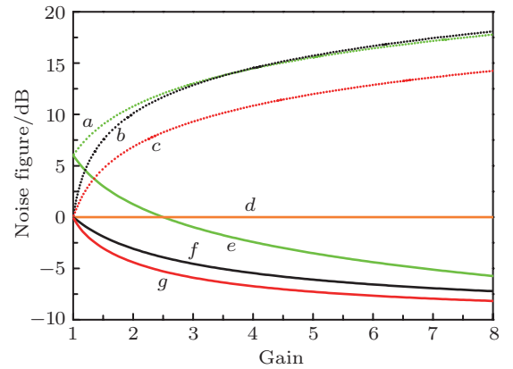
Fig. 3. (color online) Theoretical calculation of the noise figure when the losses are considered. The dotted lines correspond to the noise figure of the intensity sum, the solid orange line d is SNL, the other solid lines correspond to the noise figure of the intensity difference. Green lines a and e correspond to N_e = 3 and \eta_a = \eta_b = 1 , black lines b and f correspond to N_e = 3 , \eta_b = 0.9 when equation (20) is satisfied; red lines c and g correspond to N_e = 0 , \eta_b = 0.9 when equation (17) is satisfied.
